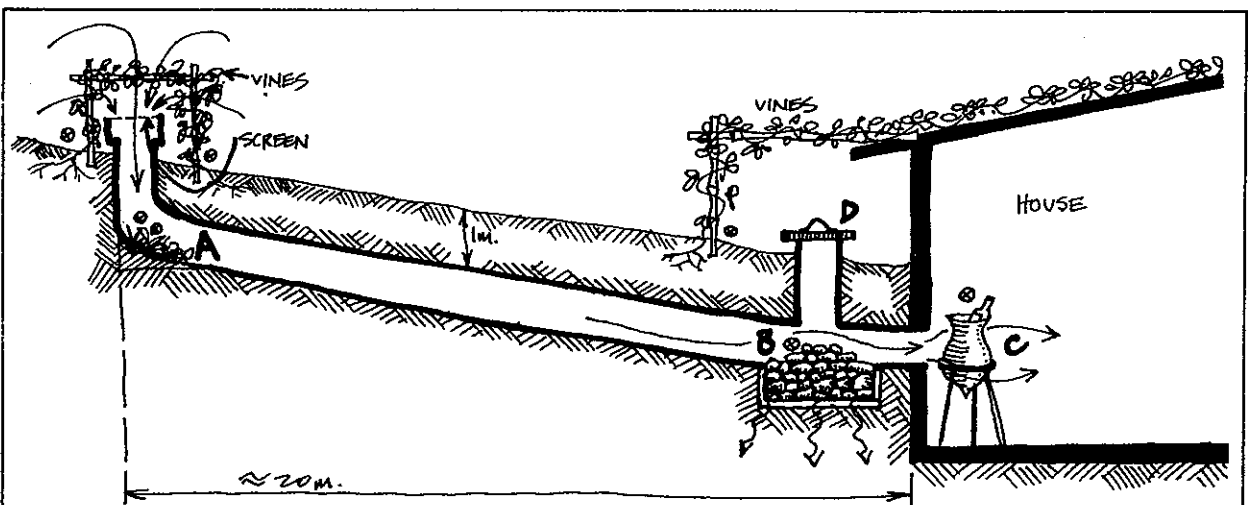
FIGURE 11.54 COOL AIR TUNNEL.
