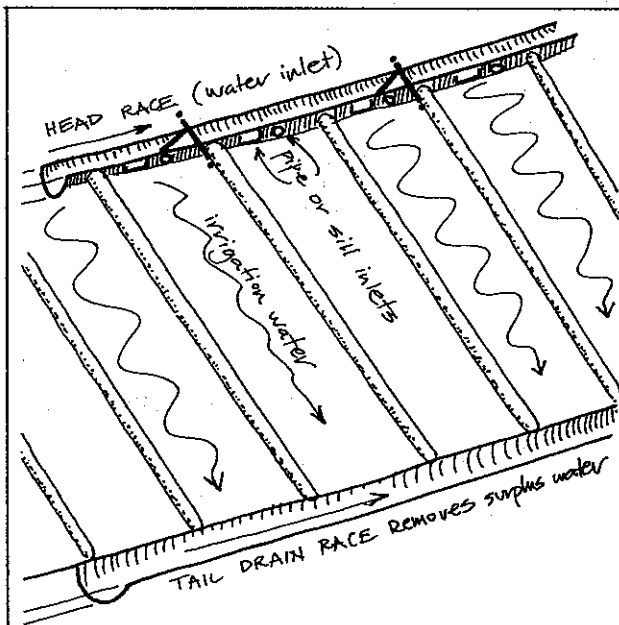
FIGURE 7.29 SCHEMATIC OF IRRIGATION BAYS
