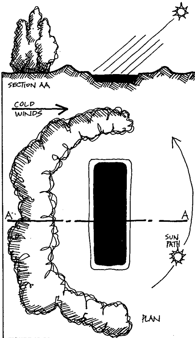
FIGURE 13.22 OXYGEN LESS IMPORTANT THAN HEATING. In cold climates, pond shelter, orientation, depth, and configuration is critical for extending warmth in cool periods, hence fish and plant growth.
