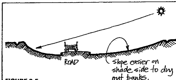
FIGURE 9.5 SLOPES CUT TO DRY OUT ROADS
