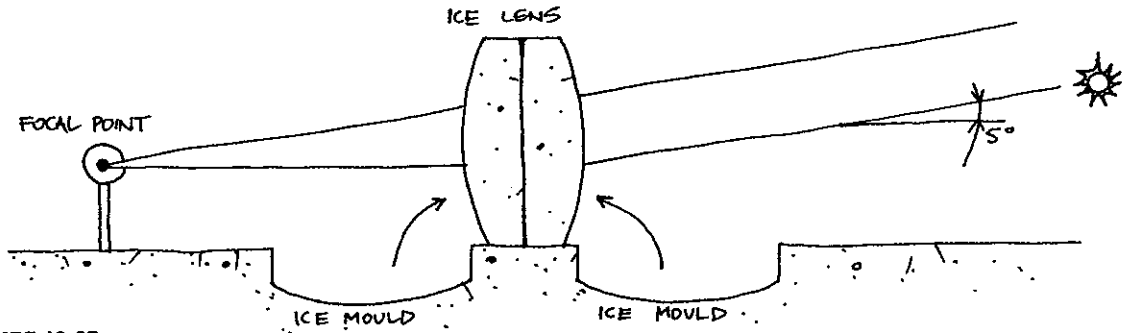
FIGURE 12.25 ICE LENSES. Ice can be moulded for use in place; here, as a focusing lens.
