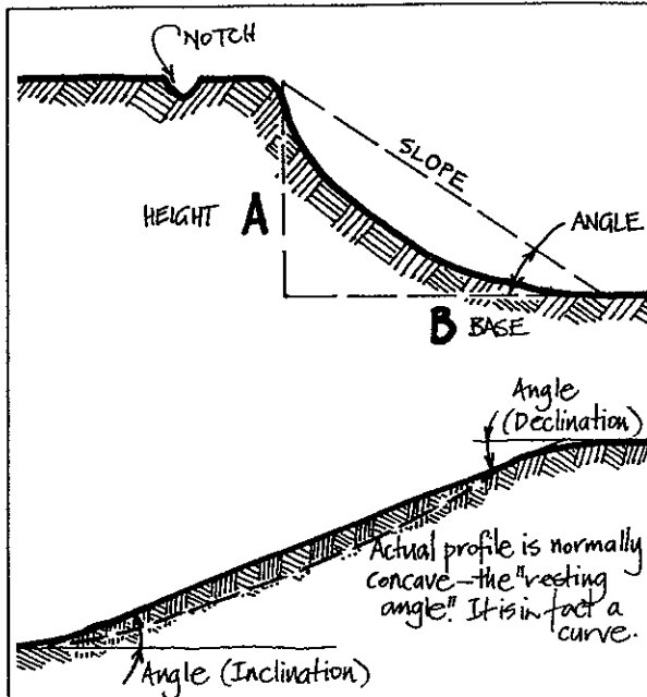
FIGURE 9.4 CONCAVE SLOPES
