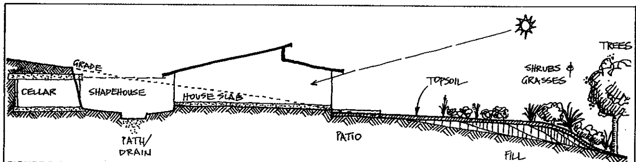
FIGURE 9.1 PREPARING A HOUSE SITE
