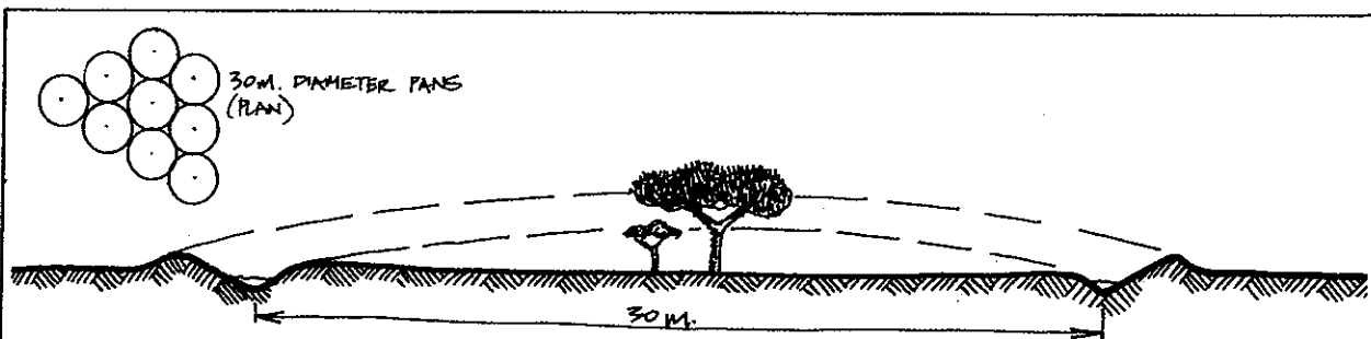
FIGURE 11.25 DITCH AND BANK LANDSCAPE IN PLAINS. Circular side-cast pans of 30 m or less diameter prevent all runoff and will grow forage species in perimeter swales; ideally, smaller (20 m or
