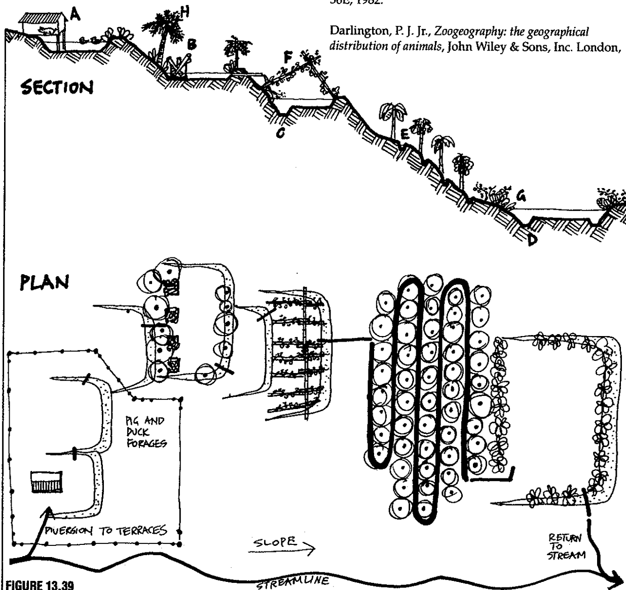
FIGURE 13.39 MODIFICATIONS TO TARO FIELDS.
