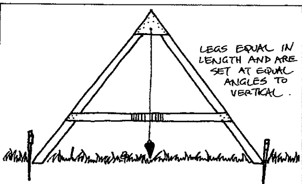
FIGURE 9.9 THE A-FRAME LEVEL About 2 m wide; legs are reversed so that plumb line cuts "level" mark on crossbeam. Used for centuries to lay out contours and drains at desired slope or flow rate.
