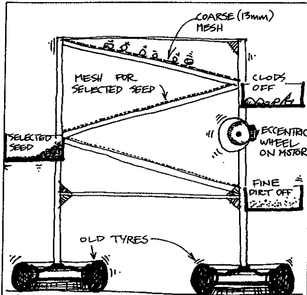
FIGURE 12.19 SEED SHAKER TRAYS. Seed from below trees is easily gathered by this electrically-operated seed shaker system; soil is simply shovelled onto the top tray.
