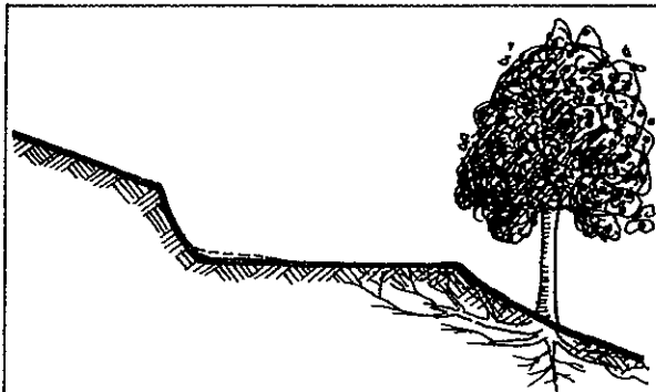
FIGURE 9.12 BENCHES CUT INTO HILLSIDES ON CONTOUR
