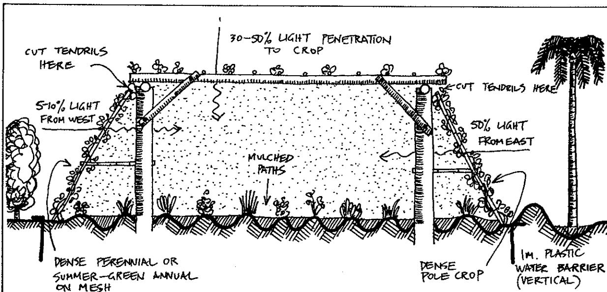
FIGURE 11.61 PLAN OF VINES OVER GARDEN.
