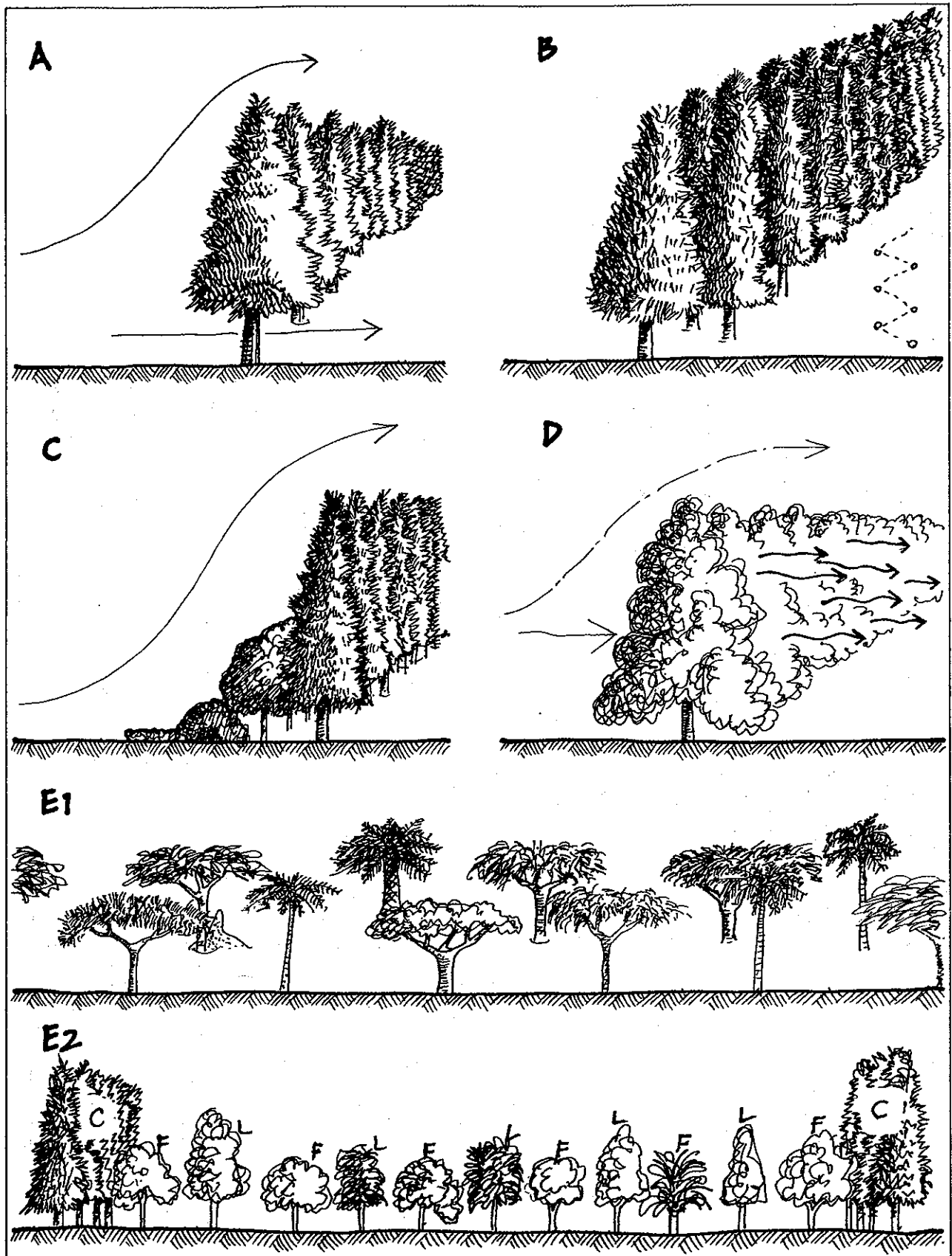
FIGURE 5.18 WINDBREAK CONFIGURATIONS.
