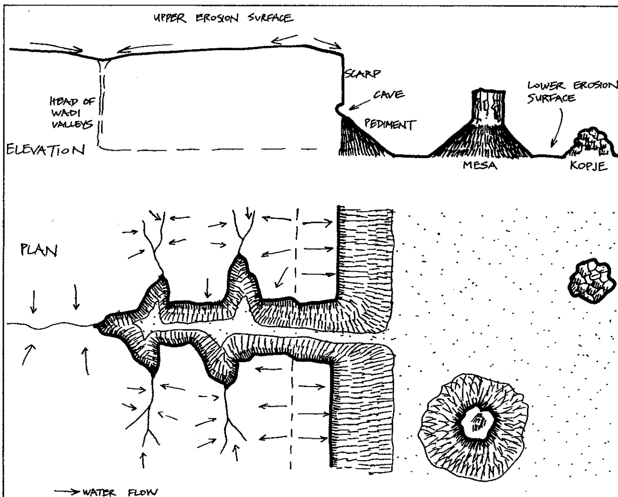
FIGURE 11.5 SCARP AND WADI DRAINAGE (Section).
