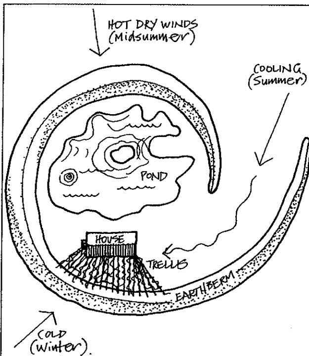
FIGURE 9.17 RAISED BANK AROUND HOUSE; this structure modifies several external climatic factors, and achieves privacy.
