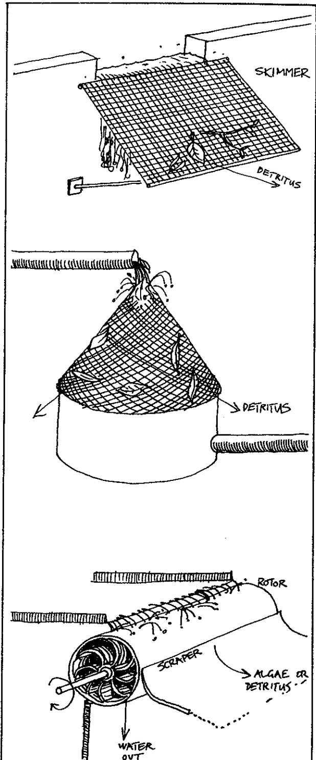
FIGURE 13.29 VARIOUS TYPES OF SCREENS to remove leaves, algae, or to self-clean.
