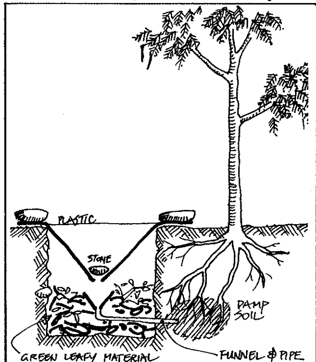
FIGURE 11.75 PIT EVAPORATION SYSTEM.
