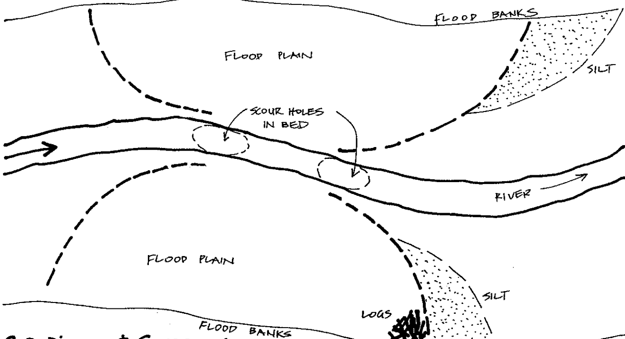
C 2. Divergent Screens. (PLAN) LEADS LOGS TO BANK AND DEPOSITS SILT ON FLOOD PLAIN. SCREENS MAY BE OF CONCRETE, ROCK WALL, OR FLOOD PLAIN TREES (IE, WILLOW OR POPLAR).
