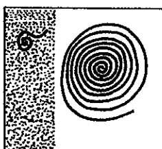
FULL MOON SHADOW AT 'MAXIMUM' RISING POINT CAST BY THIRD SLAB.
