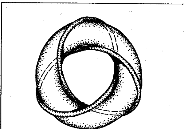
FIGURE 4.11 DNA, coiled around a plus-torus like a single path in the Robinson Congruence.
