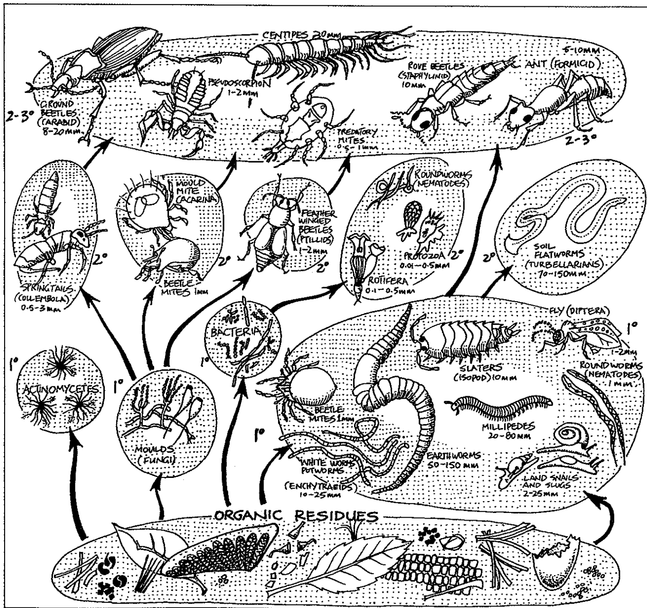
FIGURE 8.6 FOOD WEB OF A COMPOST PILE Energy flows in the direction of the arrows; lengths in millimetres. 1 = first level consumers, 2 = second level, 3 = third level.
