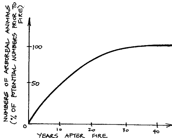
B. This curve for recovery of arboreal animals after fire could as well serve for the slow increase of fire-removed nutrients in soils and leaves.
