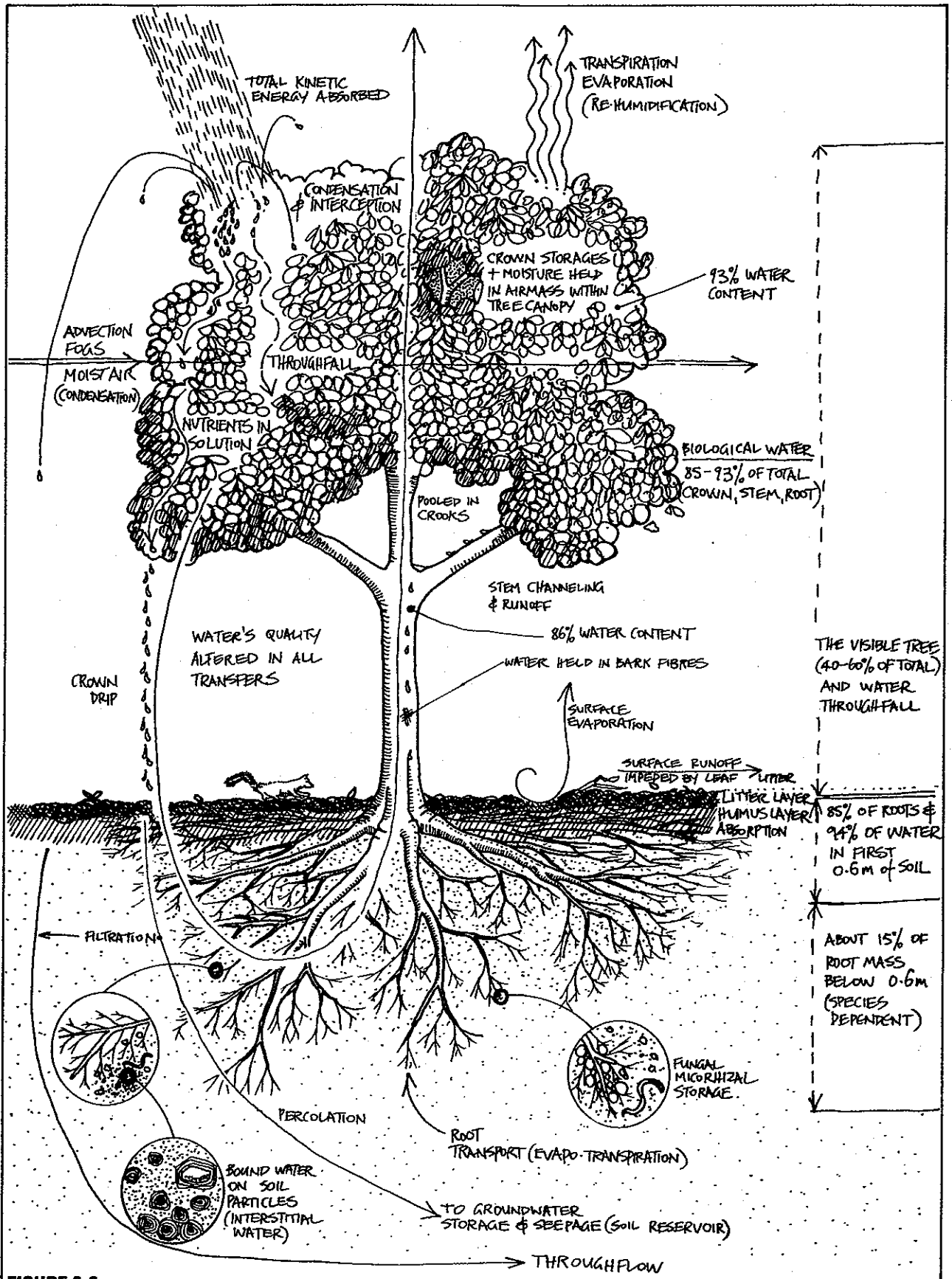
FIGURE 6.6 HOW A TREE INTERACTS WITH RAIN Every tree, every plant species, intercedes in rain to change the
