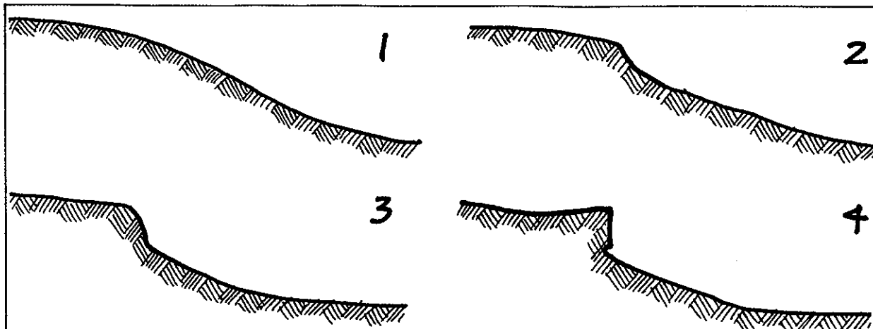
FIGURE 11.4 DEVELOPMENT OF A DESERT SCARP PROFILE.
