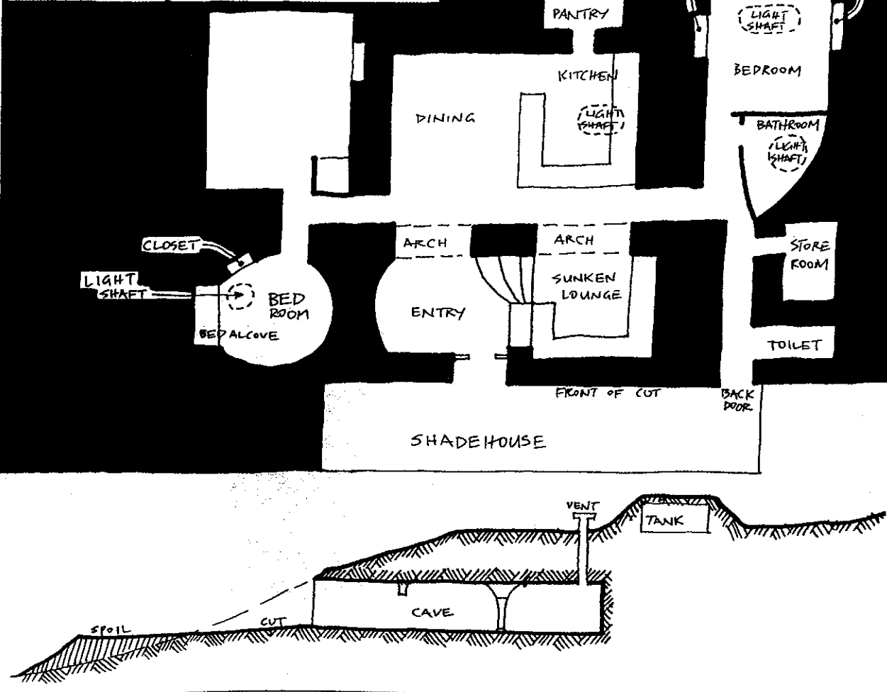
FIGURE 11.50 CAVE HOUSES (Coober Pedy, Australia). A. Vents and light shafts enable good ventilation; temperature varies 5 C annually about comfort level.
