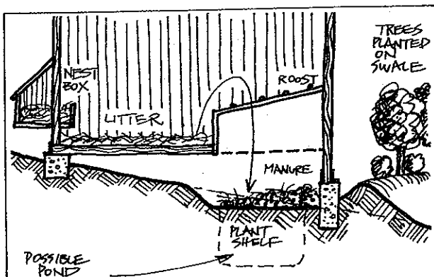
FIGURE 7.24 CHICKEN HOUSE OVER SWALE
