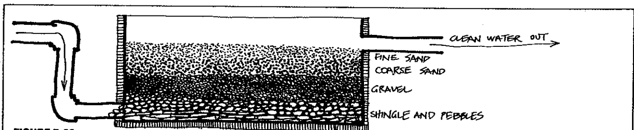
FIGURE 7.32 SAND FILTER
