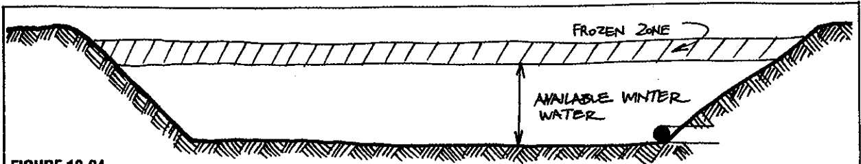
FIGURE 12.24 EXPANDING ICE IN WATER STORAGE. Sides of storages need to be sloped to allow for freeze expansion; capacity must be judged as unfrozen depth over winter.
