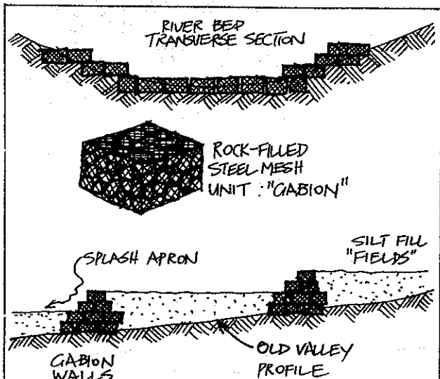
FIGURE 7.14 Eroding gullies are best stabilised using strong wire baskets to contain stones or shingle; these resist floods well.
