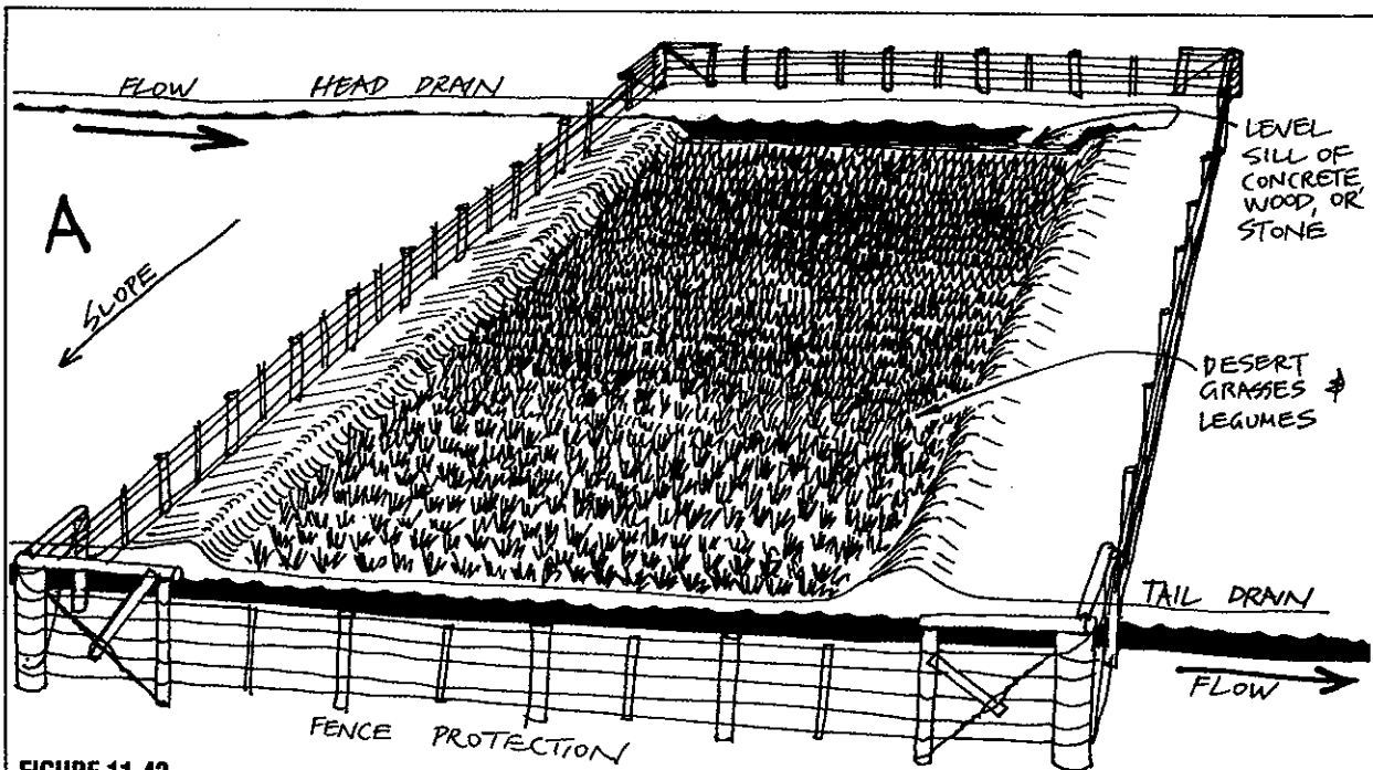
FIGURE 11.42 GRASSED SPILLWAYS WITH STEERING BANKS.
