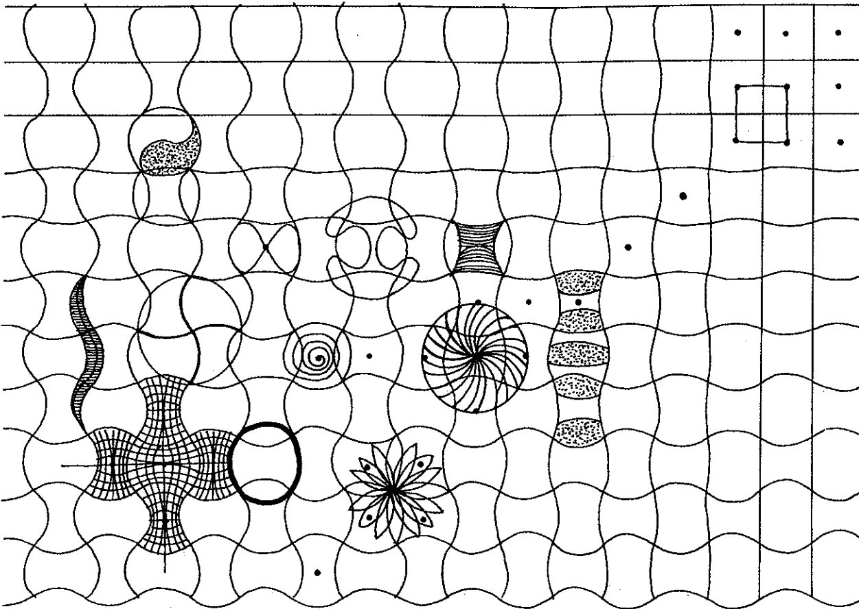
FIGURE 4. 2 PATTERN MATRIX OF TESSELLATED PATTERNS.
