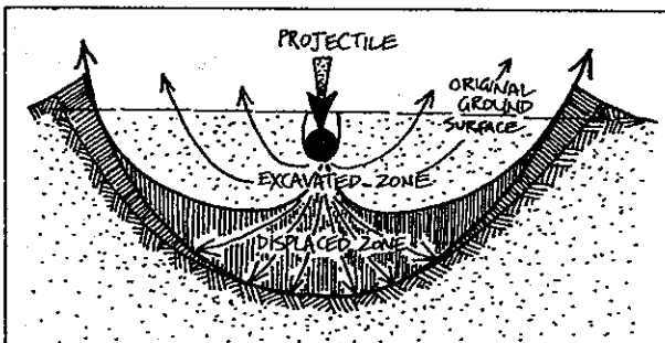
Meteor impact crater or "drip splash" forms resemble volcanic calderas.
