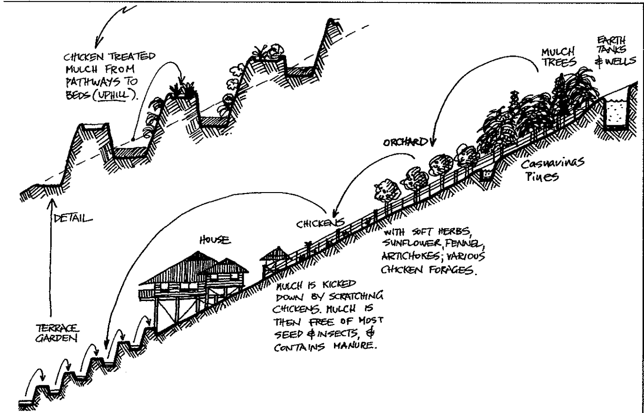
FIGURE 9.12 BENCHES CUT INTO HILLSIDES ON CONTOUR
