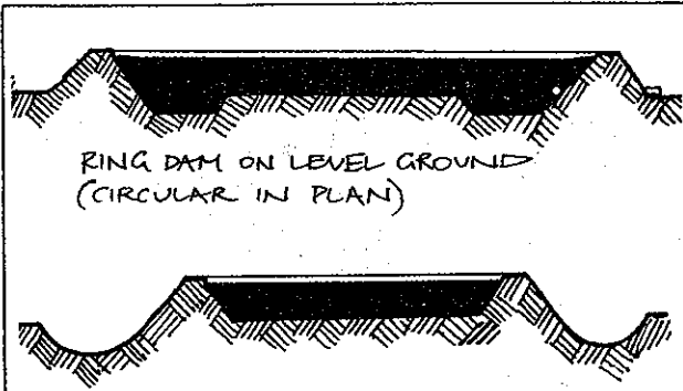
FIGURE 7.9 RING AND TURKEY'S NEST DAM. Hold water pumped in by a windmill and provides a low head in flat landscapes; can be pipe-filled from a large roof or from parking areas.
