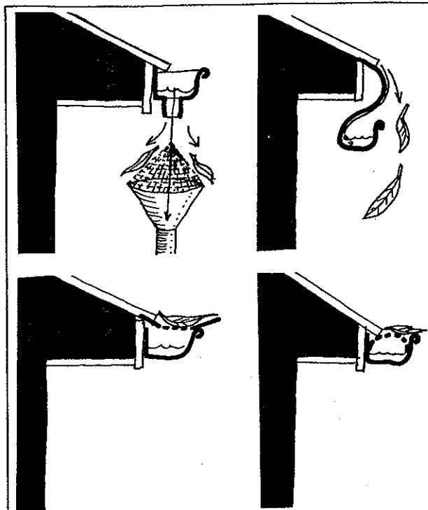
FIGURE 7.22 TYPES OF GUTTERS
