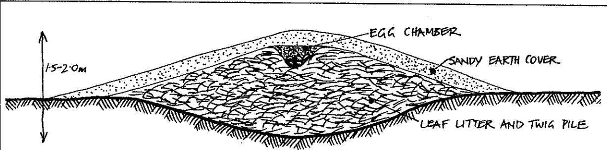
FIGURE 11.83 MALLEE FOWL NEST. A. In effect, a compost heap. Pack rats and stick nest rats also make large nests in drylands; if we duplicate this structure, water held in the heap enables trees more suited to rainforest to be planted if rainforest soils are used in nurseries. B. Swale base can have a variety of "furniture" or trials of special niches for trees and water retention.
