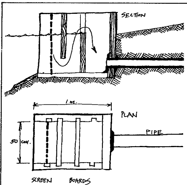
FIGURE 13.28 SCREENS AND BOARDS. Classical "Herguth monk" outlet incorporates a screen and a level control board.
