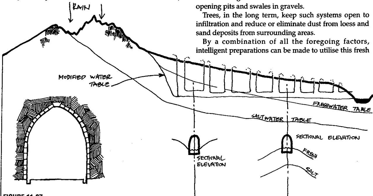
FIGURE 11.37 QUANATS.
