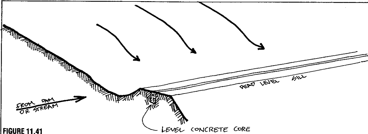
FIGURE 11.41 VERY LONG SPREADER BANKS.
