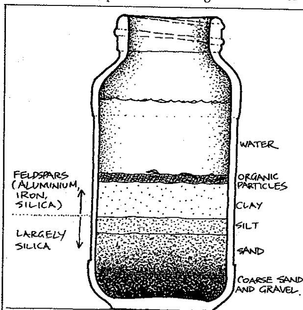
FIGURE 8.2 JAR METHOD
