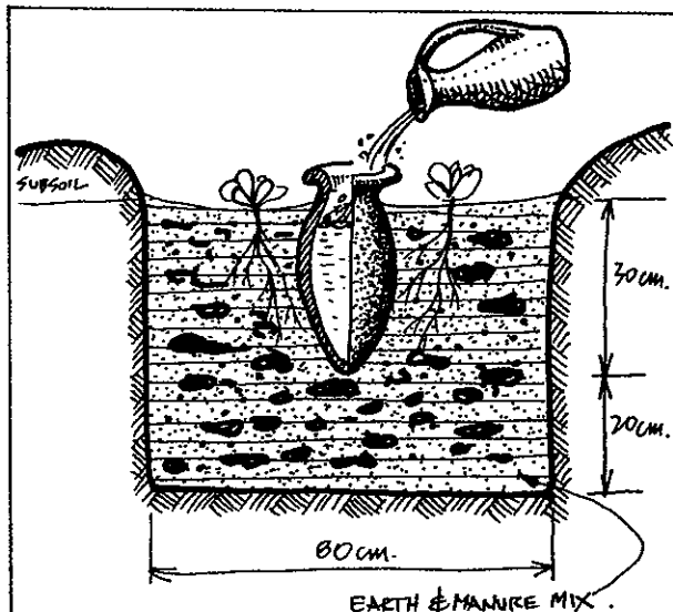
FIGURE 11.69 POT SYSTEM.
